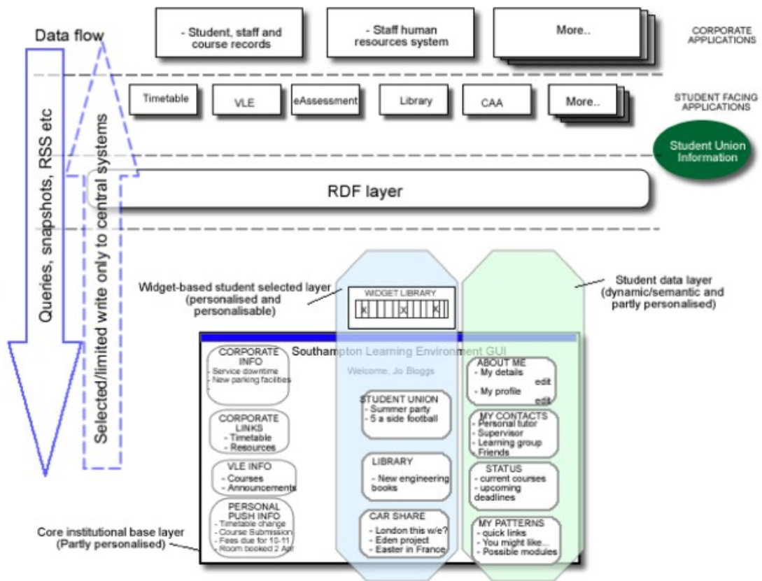
Figure 4: Proposed SLE Architecture showing personalised widget/portal front-end to SLE and the existing student facing applications and enterprise DBs.
